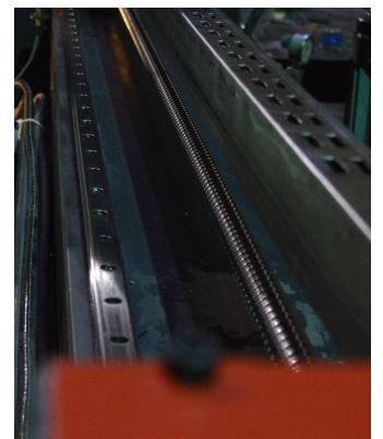
Feeding, Through, LM Guides and Ball Screw
